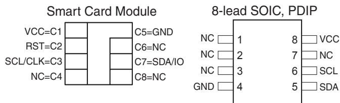
Figure 1. Package Options
