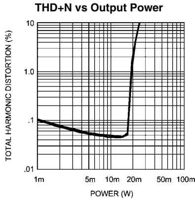
200486g7 Analog V_{DD} = 2.6V , Digital V_{DD} = 2.6V R_L = 32\Omega , 44.1 kHz Sample Rate R & L Channels Shown, Vol = 3dB, Frequency in = 1kHz
