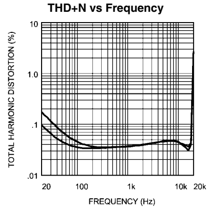
200486g6 Analog V_{DD} = 5V , Digital V_{DD} = 3V R_L = 32\Omega , Power Level = 50mW R & L Channels Shown, 44.1kHz Sample Rate
