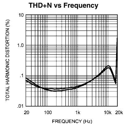
200486g4 Analog V_{DD} = 2.6V , Digital V_{DD} = 2.6V R_L = 32\Omega , Power Level = 12mW R & L Channels Shown, 44.1kHz Sample Rate
