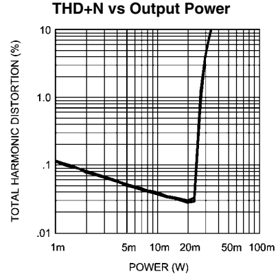
200486g8 Analog V_{DD} = 3V , Digital V_{DD} = 3V R_L = 32\Omega , 44.1 kHz Sample Rate R & L Channels Shown, Vol = 3dB, Frequency in = 1kHz
