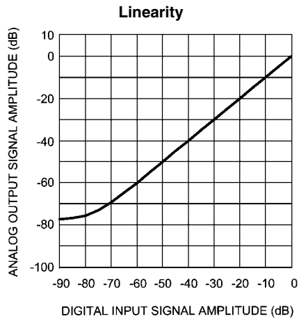
200486e3 Analog V_{DD} = 5V , Digital V_{DD} = 3V R_L = 32\Omega , 44.1kHz Sample Rate
