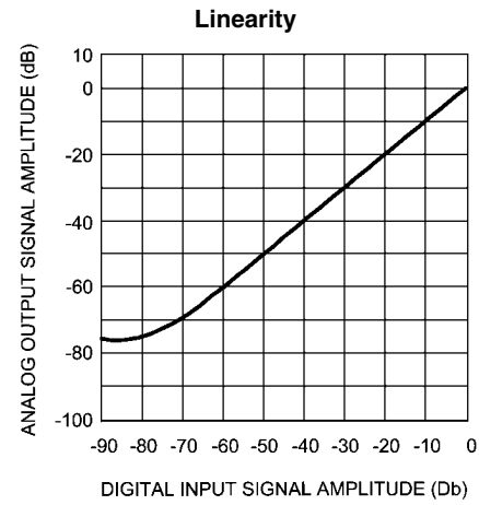
200486e2 Analog V_{DD} = 3V , Digital V_{DD} = 3V R_L = 32\Omega , 44.1kHz Sample Rate
