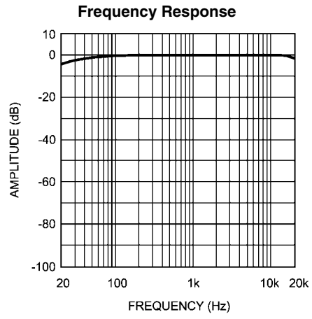
200486e1 Analog V_{DD} = 5V , Digital V_{DD} = 3V R_L = 32\Omega , Vol = 0dB 44.1kHz Sample Rate, 0dB FFS
