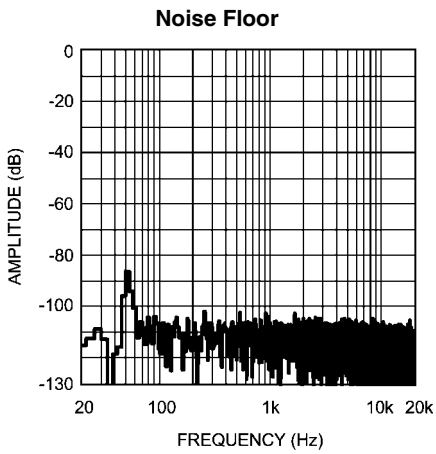
200486f0 Analog V_{DD} = 5V , Digital V_{DD} = 3V R_L = 32\Omega , Vol = 3dB, 44.1kHz Sample Rate
