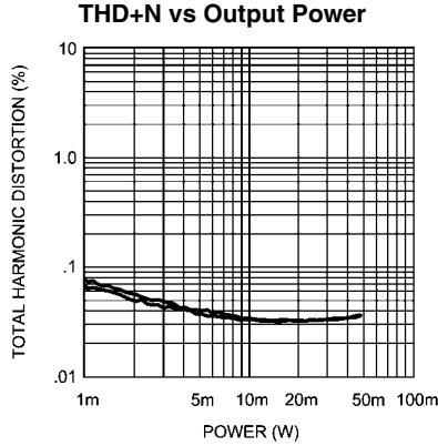
200486g9 Analog V_{DD} = 5V , Digital V_{DD} = 3V R_L = 32\Omega , 44.1 kHz Sample Rate R & L Channels, Vol = 3dB, Frequency in = 1kHz
