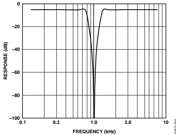
Figure 2. Band-Reject Response
