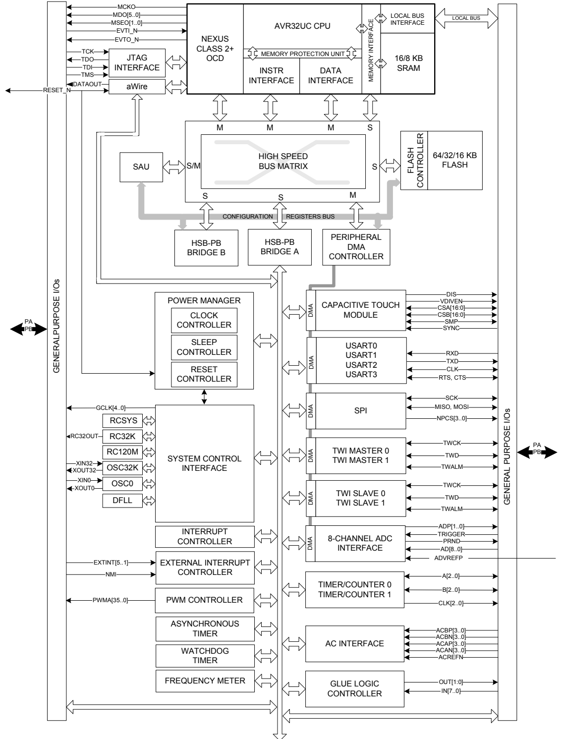
Figure 2-1. Block Diagram
