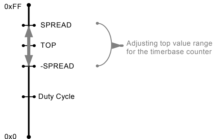
Figure 23-2. PWMA Adjusting Top Value for Timebase Counter
