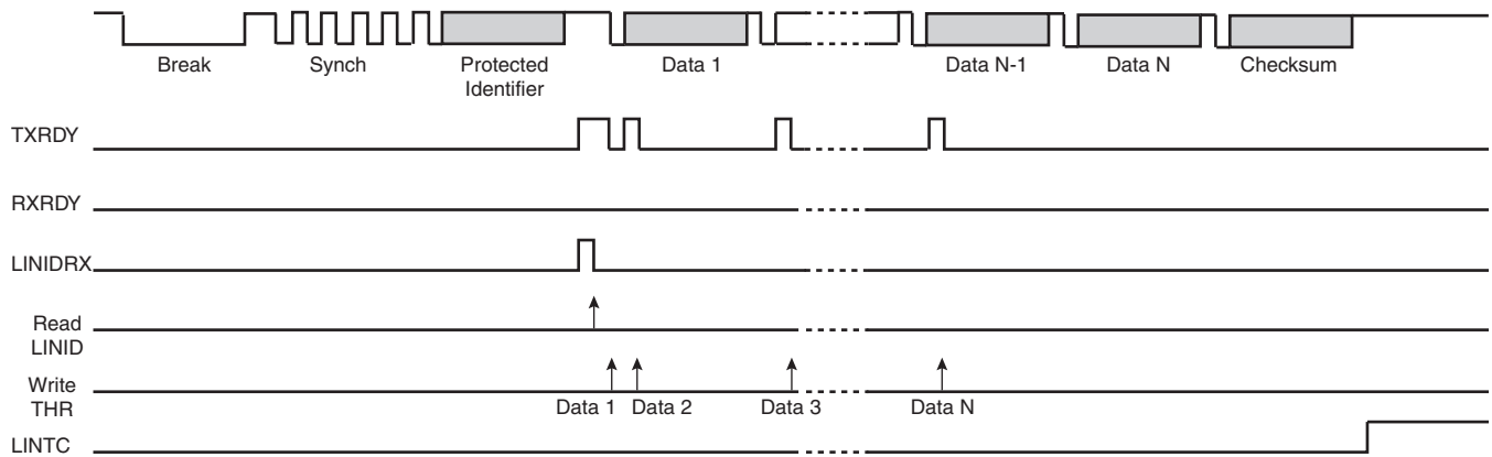
Figure 19-30. Slave Node Configuration, NACT=PUBLISH
