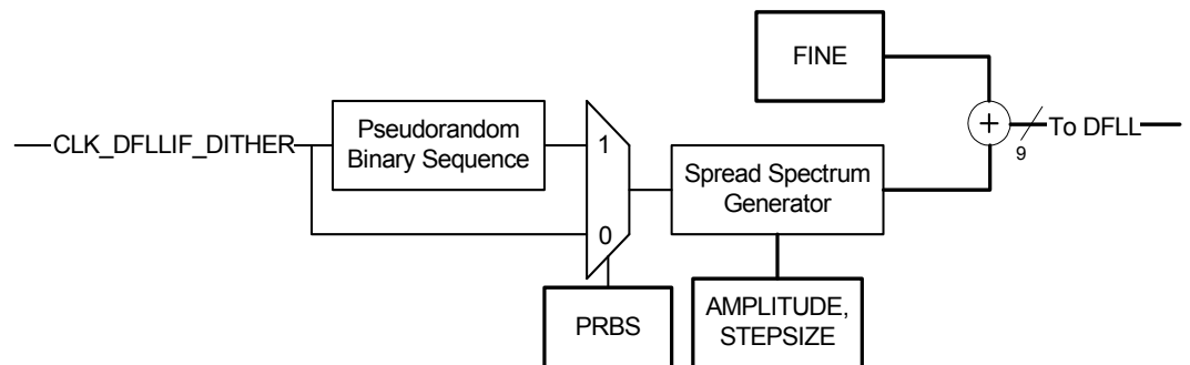
Figure 13-4. Spread Spectrum Generator Block Diagram.
