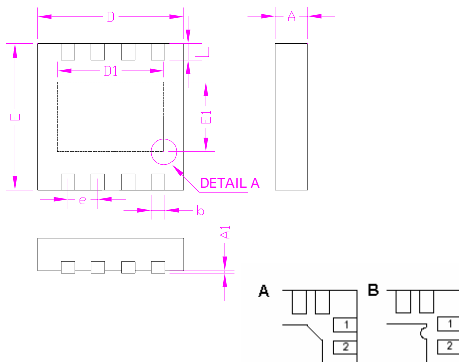
DETAIL A Thermal Pad Option
