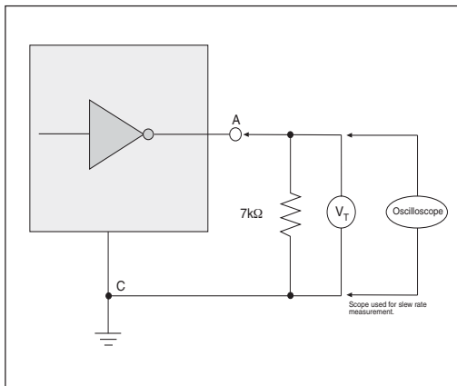
Figure 14. V.28 Driver Output Slow Rate
