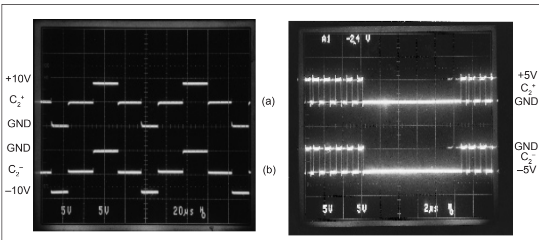
Figure 18a and 18b. Charge Pump Waveform
