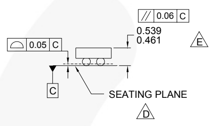
SIDE VIEWS
