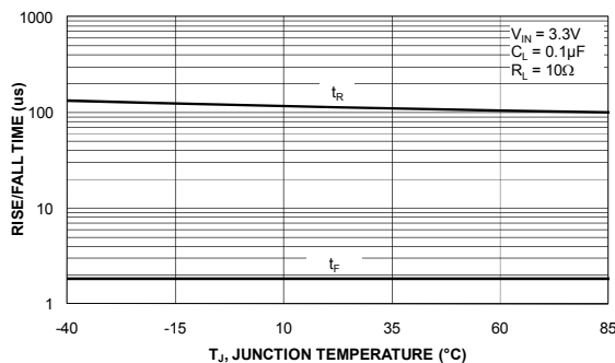
Figure 16. V_{OUT} Rise and Fall Time vs. Temperature at R_L=10\Omega
