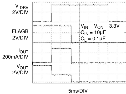
Figure 17. T_{BLANK} Response
