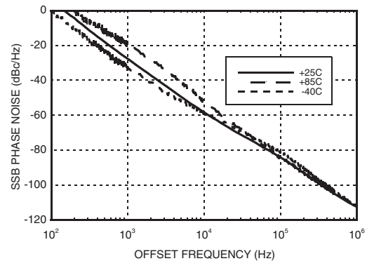
Typical SSB Phase Noise @ Vtune = +12V
