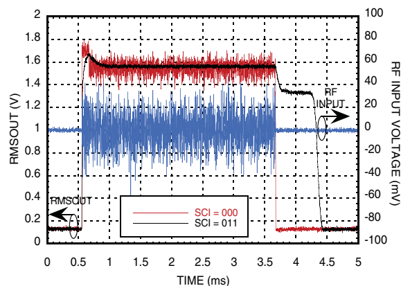
Residual Ripple for 0.9 GHz WiBRO @ SCI = 101
