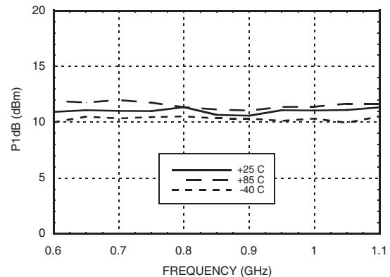
Single Channel: Input P1dB vs. Temperature
