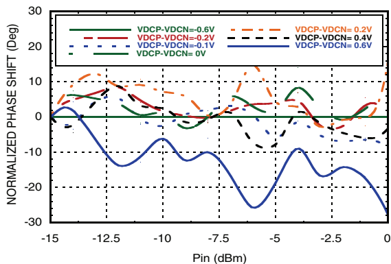
Phase Shift vs. Control Voltage @ 22 GHz [1][2][3][4]
