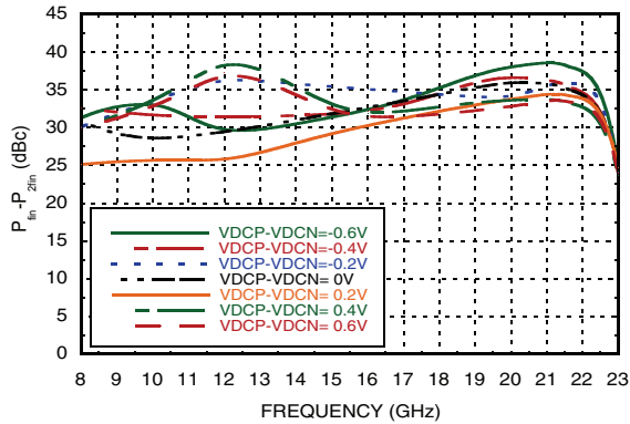
Second Harmonic vs. Control Voltage [1][2]
