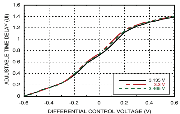
Time Delay vs. Bias Voltage [2][3][4]
