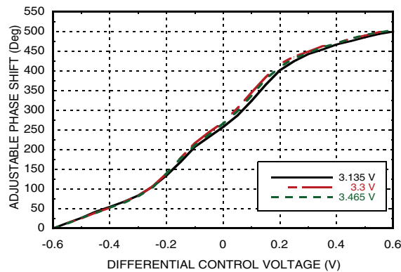
Phase Shift vs. Bias Voltage [2][3][4]
