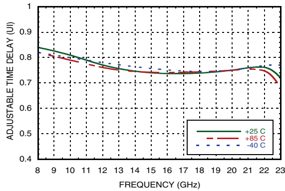
Time Delay vs. Temperature @ VDCP=3.3V (Relative to VDCP=VCC-0.6V) [1][2][6]
