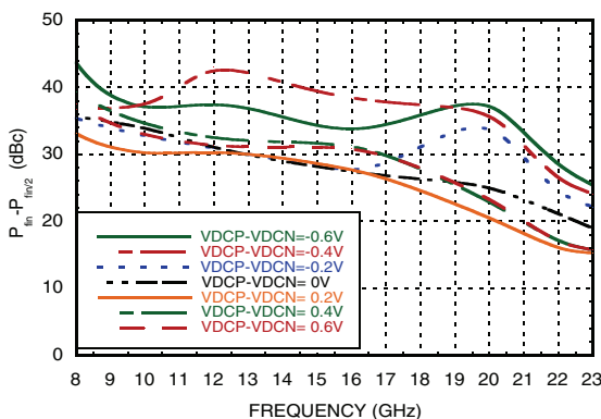
P_{in} - P_{fin/2} Output Power Difference vs. Control Voltage [1][2][5]
