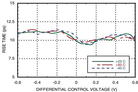
Rise Time vs. Temperature @ 16 GHz [1][2][3]
