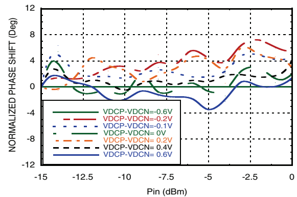
Phase Shift vs. Control Voltage @ 10 GHz [1][2][3][4]
