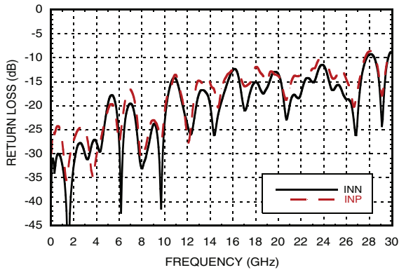
Input Return Loss vs. Frequency [1][4]
