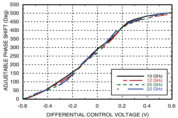
Phase Shift vs. Frequency [1][2][3]
