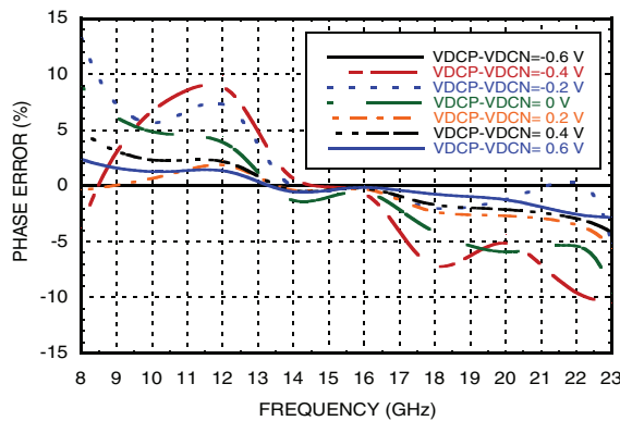
Phase Error vs. Control Voltage @ f_{mean}=16 GHz [1][2][3][4]
