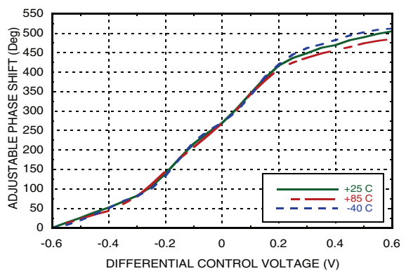
Phase Shift vs. Temperature [1][2][3][4]
