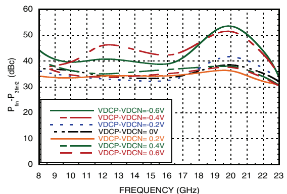
P_{in} - P_{3fin/2} Output Power Difference vs. Control Voltage [1][2][5]
