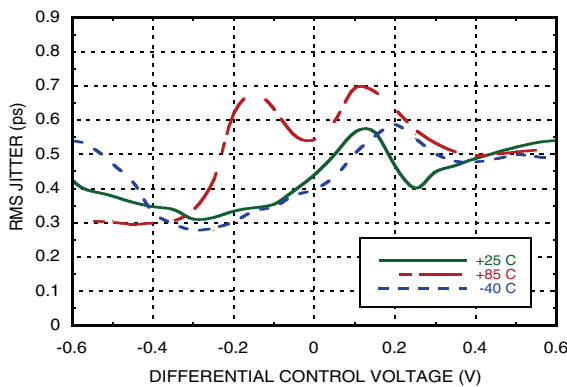
RMS Jitter vs. Temperature @ 16 GHz [1][2][3][4]
