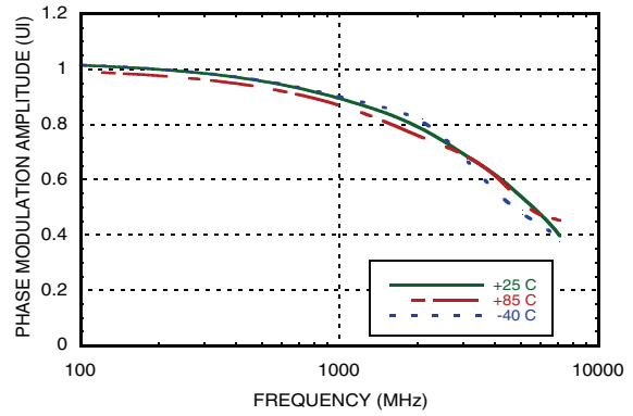
Modulation Signal Bandwidth vs. Temperature [1][3]
