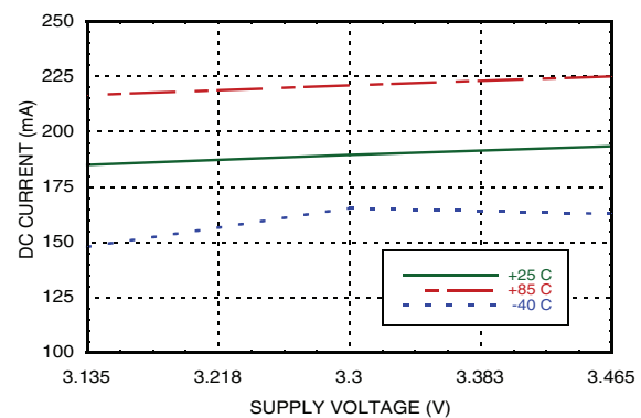
DC Current vs. Temperature [2][5]
