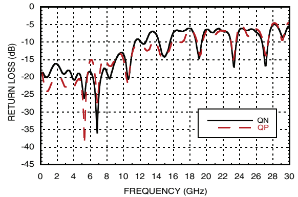
Output Return Loss vs. Frequency [1][4]
