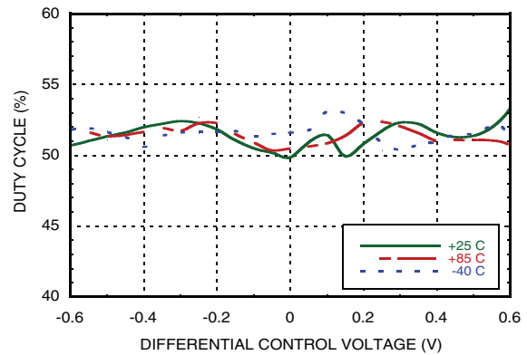
Duty Cycle Distortion @ 16 GHz [1][4][5]
