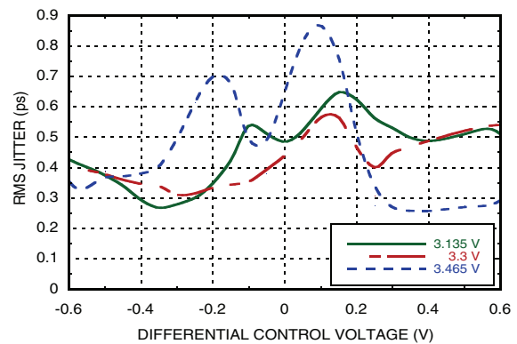
RMS Jitter vs. Bias Voltage @ 16 GHz [1][3][4]
