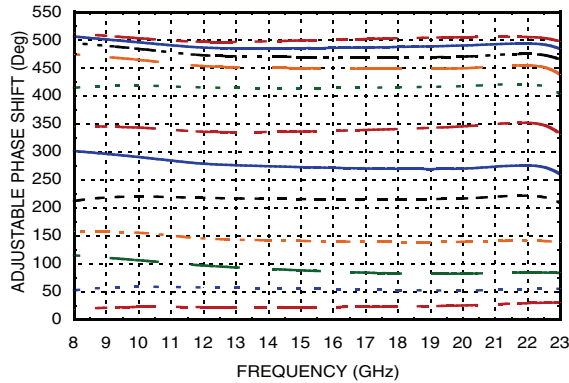
Phase Shift vs. Control Voltage @ V_{DCP}=2.7V to 3.9V with 0.1V step [1][2][3]
