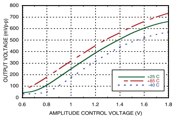
Single-Ended Output Swing vs. Amplitude Control Voltage [1][3][4][6]
