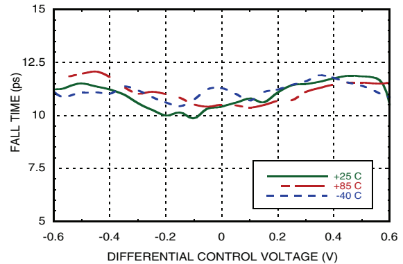
Fall Time vs. Temperature @ 16 GHz [1][2][3]
