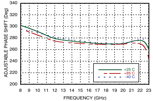
Phase Shift vs. Temperature @ V_{DCP}=3.3V (Relative to V_{DCP}=V_{CC}-0.6V ) [1][2]
