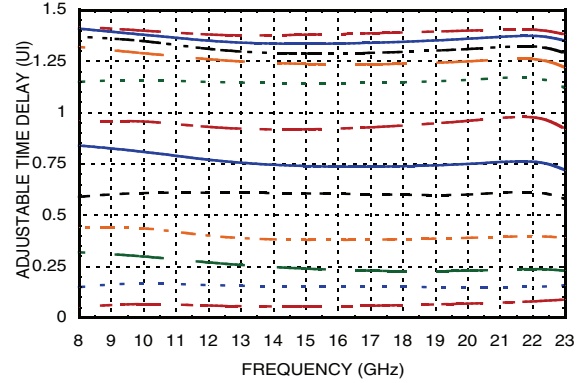
Time Delay vs. Control Voltage @ VDCP=2.7V to 3.9V with 0.1V step [1][2]
