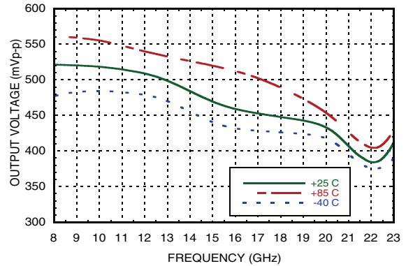
Single-Ended Output Swing vs. Frequency [1][3][4]
