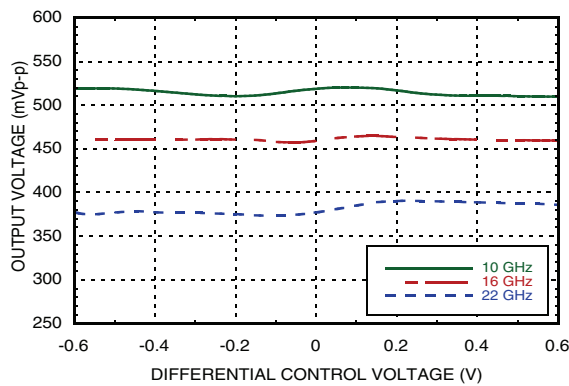
Single-Ended Output Swing vs. Control Voltage [1][4][5]
