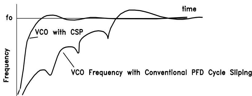
Figure 30. Cycle Slipping
