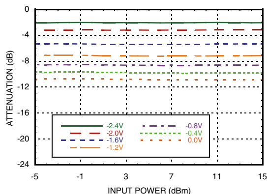
Attenuation vs. Pin @ 20 GHz over Vctrl1 Vctrl1 = Variable, Vctrl2 = -3V
