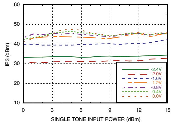
Input IP3 vs. Input Power Over Vctrl @ 20 GHz, Vctrl1 = Vctrl2
