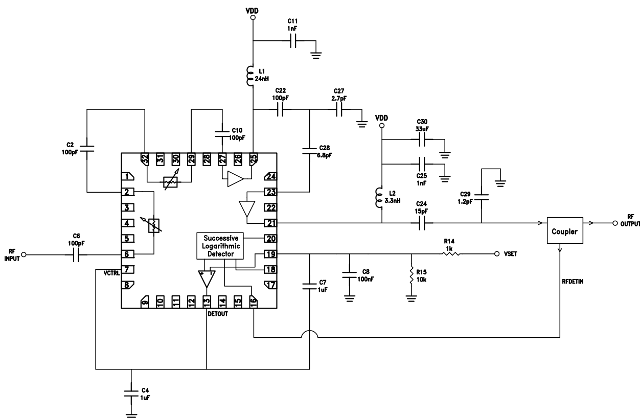
Figure 5: The HMC993LP5E's AGC configuration with 2 attenuators, 1900 MHz tune.
