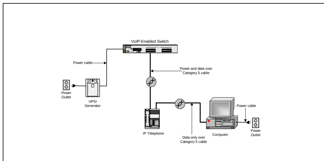
Figure 30. Typical IP Telephone System Connection
