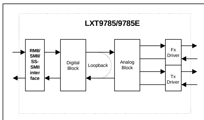
Figure 9. Internal Loopback
