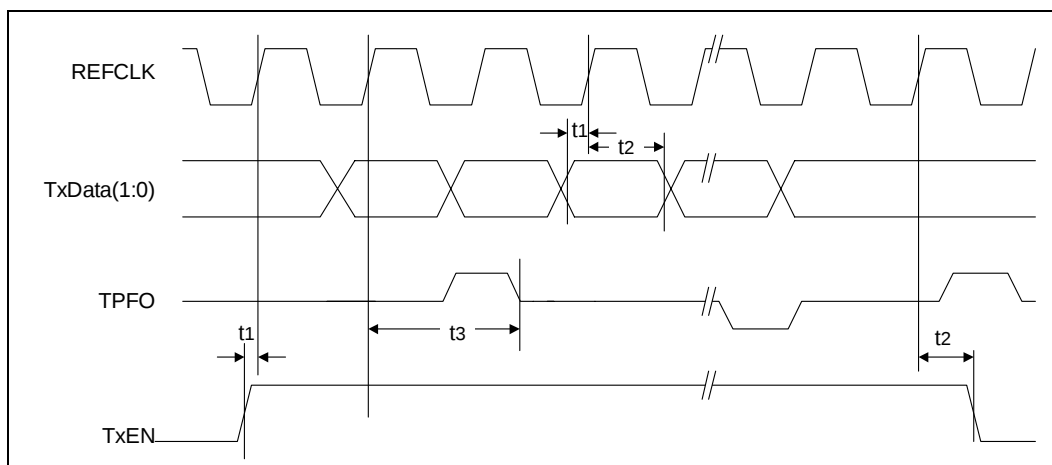
Figure 53. RMII - 100BASE-FX Transmit Timing
