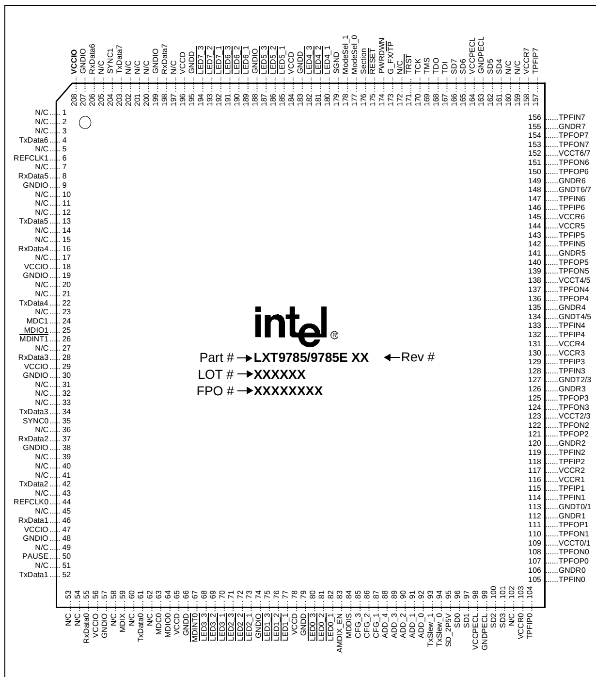
Figure 3. LXT9785/9785E SMII 208-Pin PQFP Assignments
