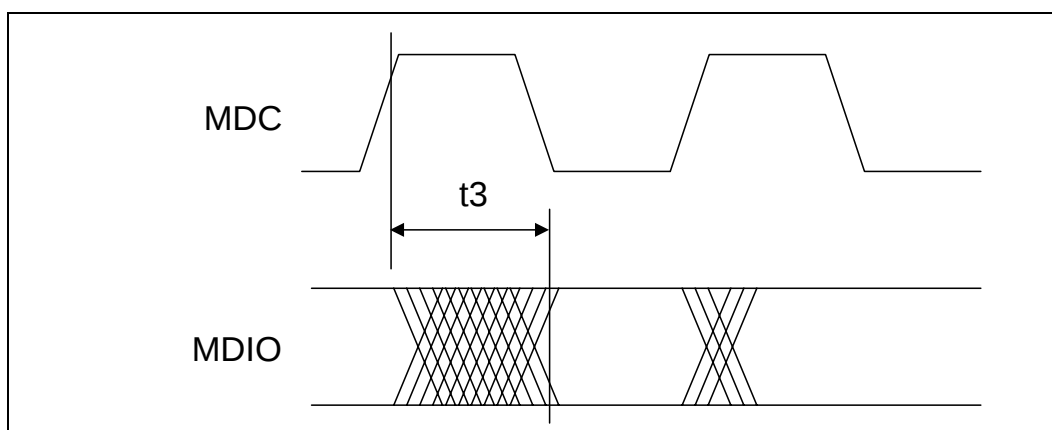
Figure 59. MDIO Read Timing (MDIO Sourced by PHY)
