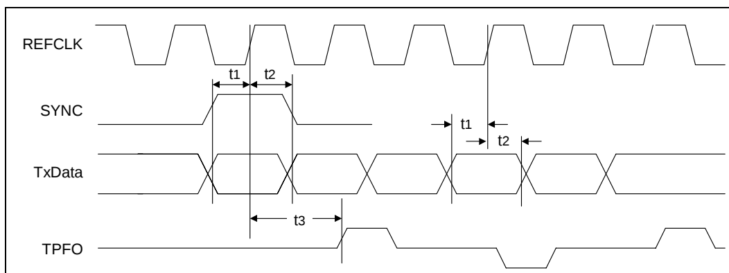
Figure 41. SMI - 100BASE-FX Transmit Timing
