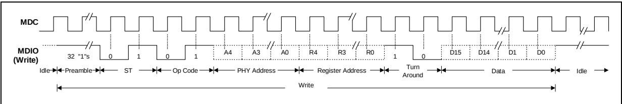
Figure 11. Management Interface Write Frame Structure
