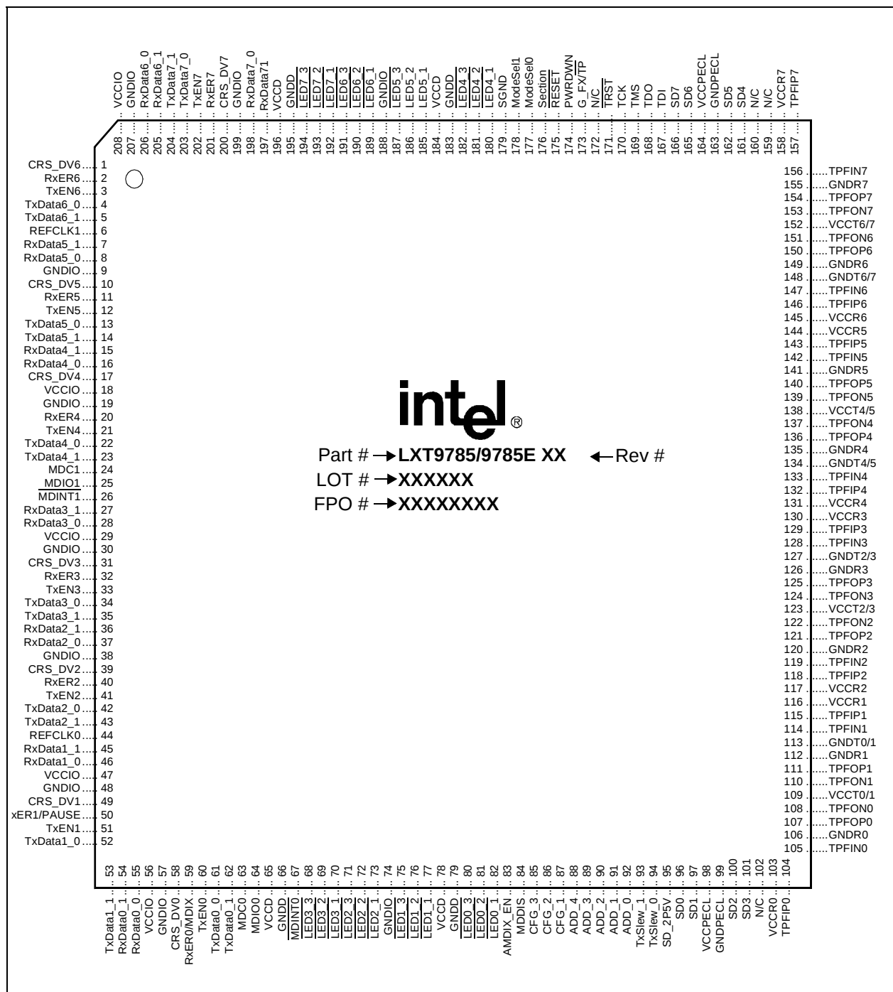
Figure 2. LXT9785/9785E RMII 208-Pin PQFP Assignments
