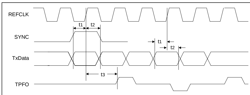
Figure 43. SMII - 10BASE-T Transmit Timing
