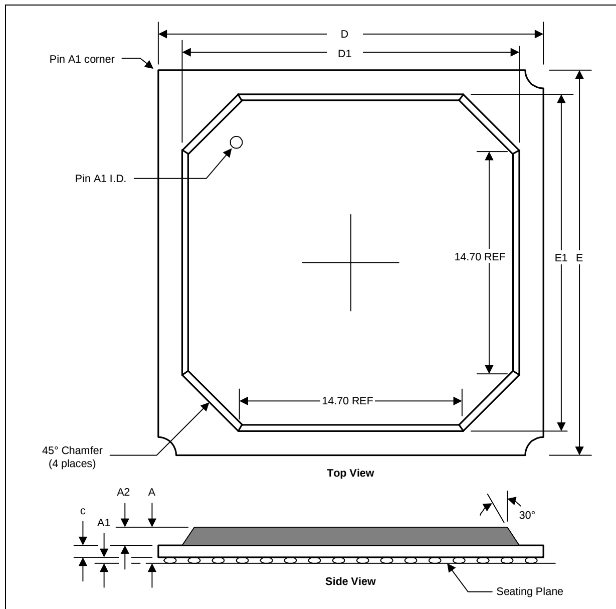
Figure 64. LXT9785/9785E 241-Ball PBGA Package Specs - Top/Side View(LXT9785BC/ LXT9785EBC)
