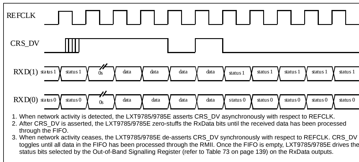
Figure 33. RMII Programmable Out-of-Bank Signaling
