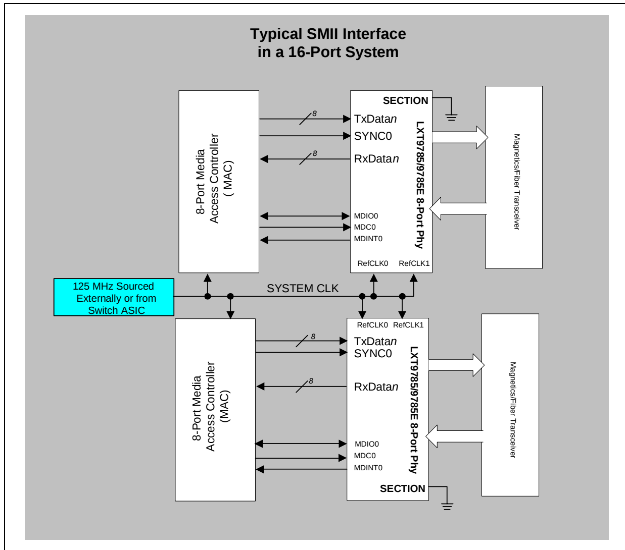
Figure 16. Typical SMI Interface Diagram
