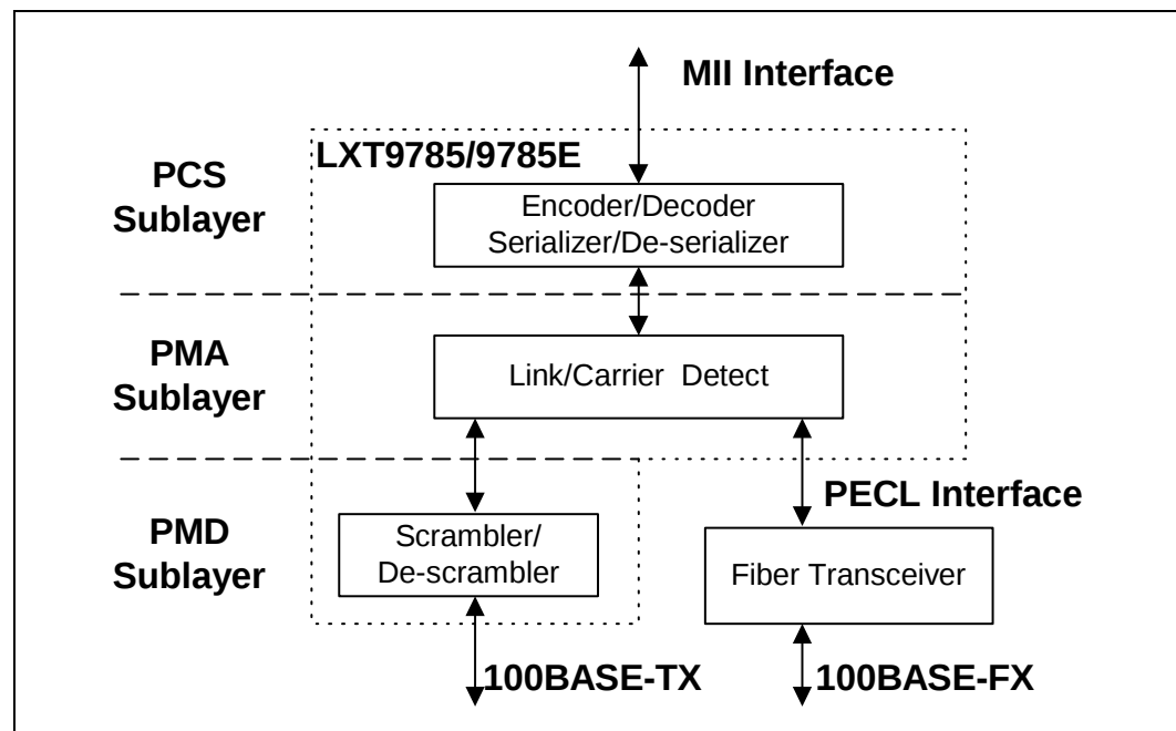
Figure 29. Protocol Sublayers
