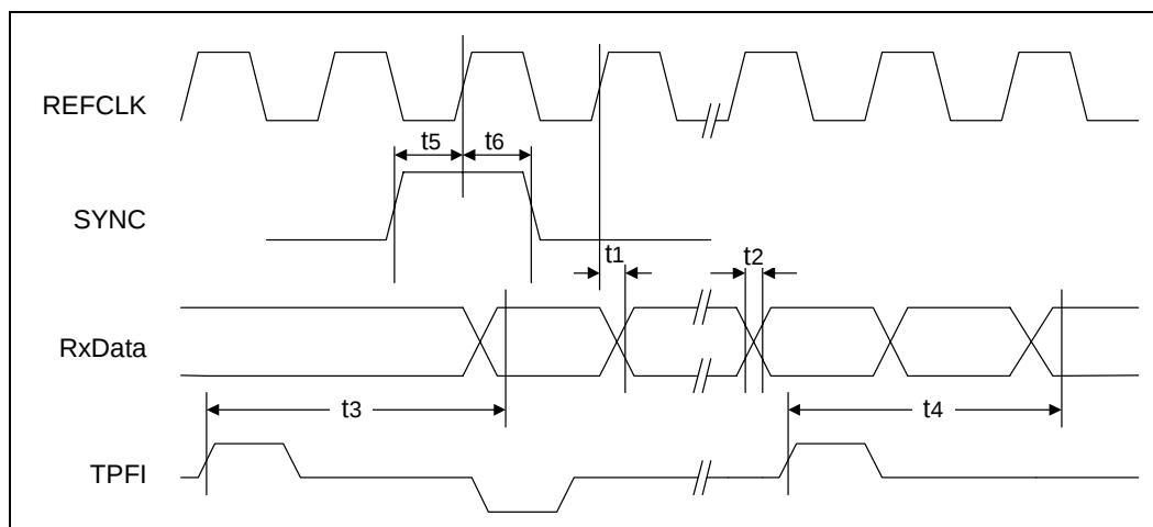
Figure 38. SMII - 100BASE-TX Receive Timing
