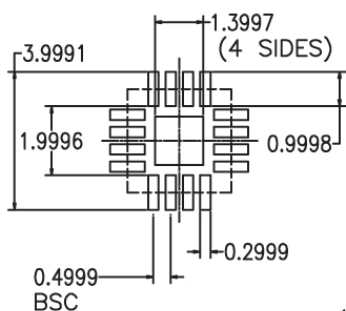
RECOMMENDED SOLDER PAD PITCH AND DIMENSIONS
