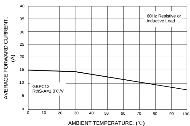
FIG. 2 - MAXIMUM OUTPUT RECTIFIED CURRENT
