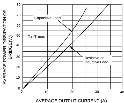
FIG. 3- MAXIMUM POWER DISSIPATION
