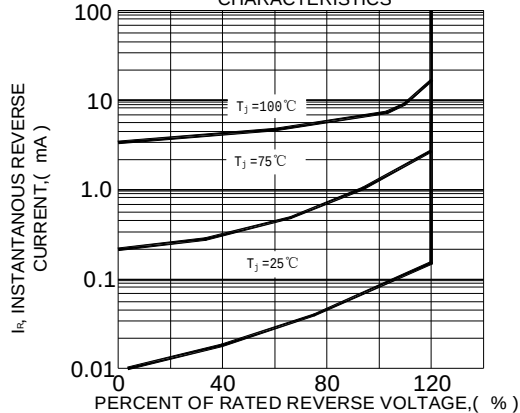
FIG.5-TYPICAL REVERSE CHARACTERISTICS
