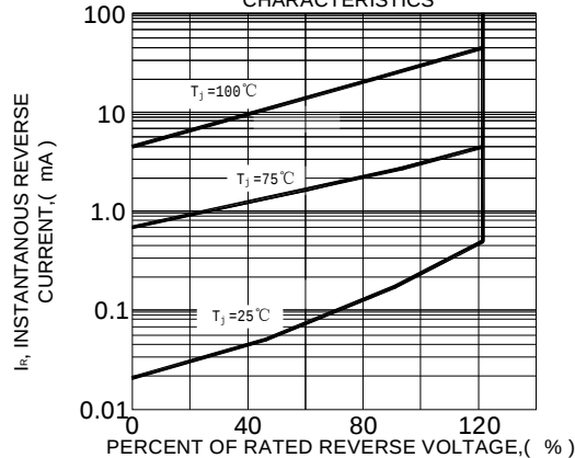
FIG.5-TYPICAL REVERSE CHARACTERISTICS
