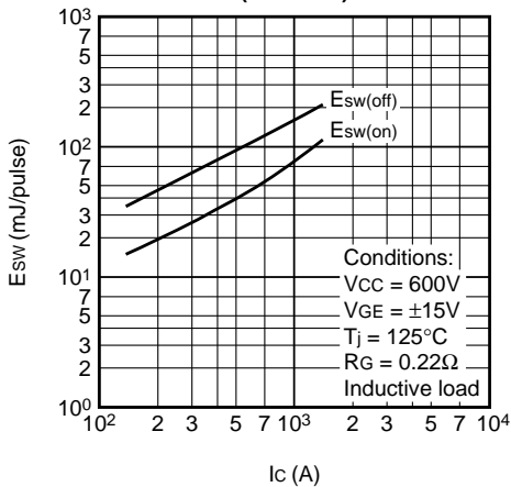
Ic-Esw (TYPICAL)
