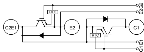
CIRCUIT DIAGRAM
