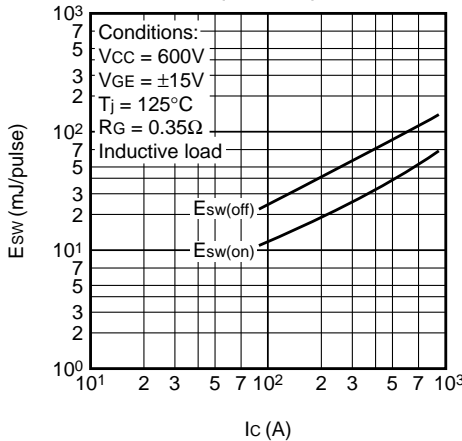
Ic-Esw (TYPICAL)
