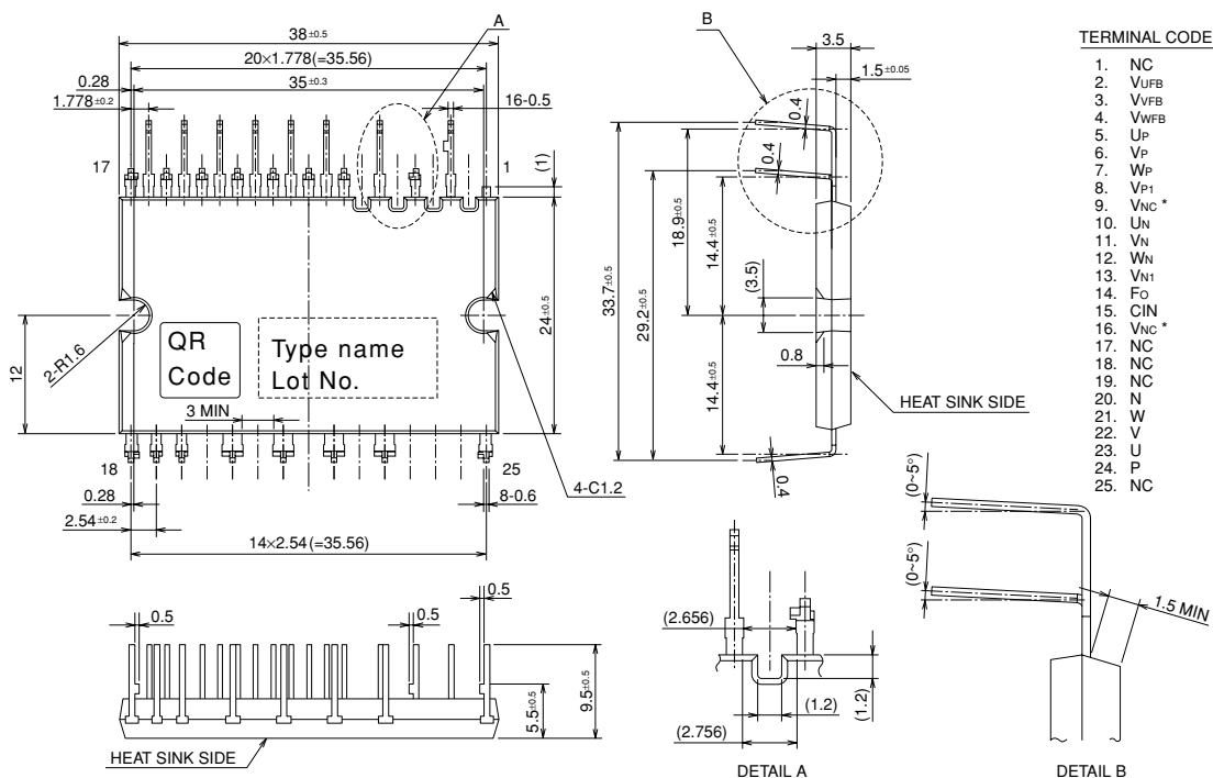
Fig. 3 ZIGZAG TERMINAL TYPE PACKAGE OUTLINES (PS21961-CT)
