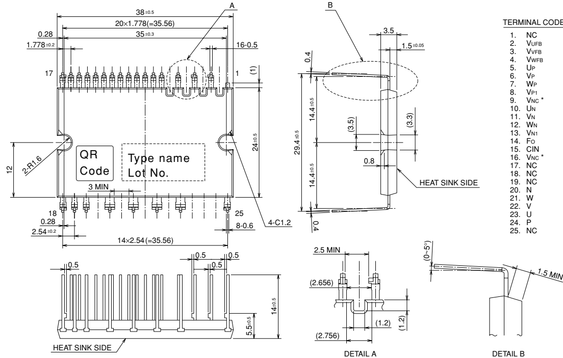
Fig. 2 LONG TERMINAL TYPE PACKAGE OUTLINES (PS21961-AT)
