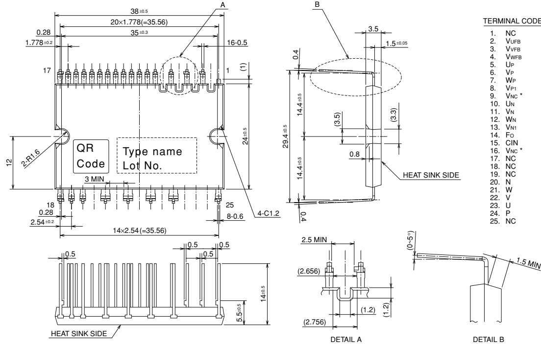
Fig. 2 LONG TERMINAL TYPE PACKAGE OUTLINES (PS21962-4A)
