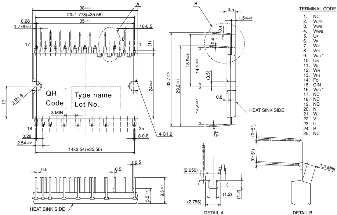
Fig. 3 ZIGZAG TERMINAL TYPE PACKAGE OUTLINES (PS21962-4C)
