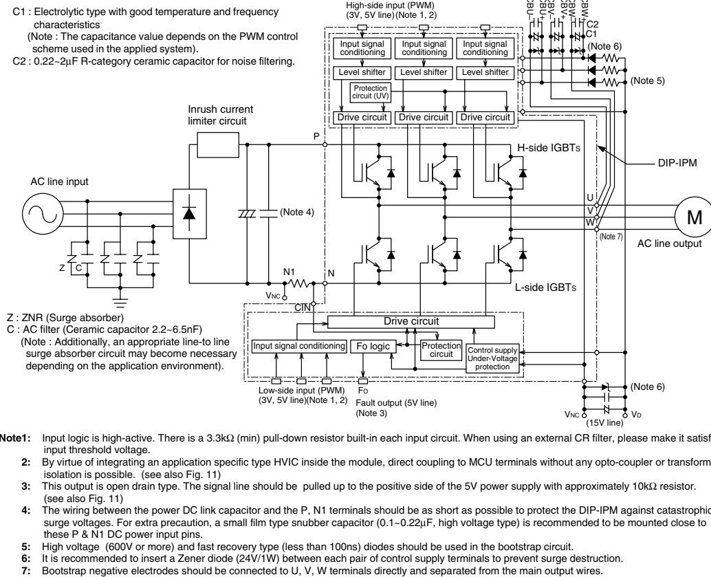
Fig. 5 INTERNAL FUNCTIONS BLOCK DIAGRAM (TYPICAL APPLICATION EXAMPLE)
