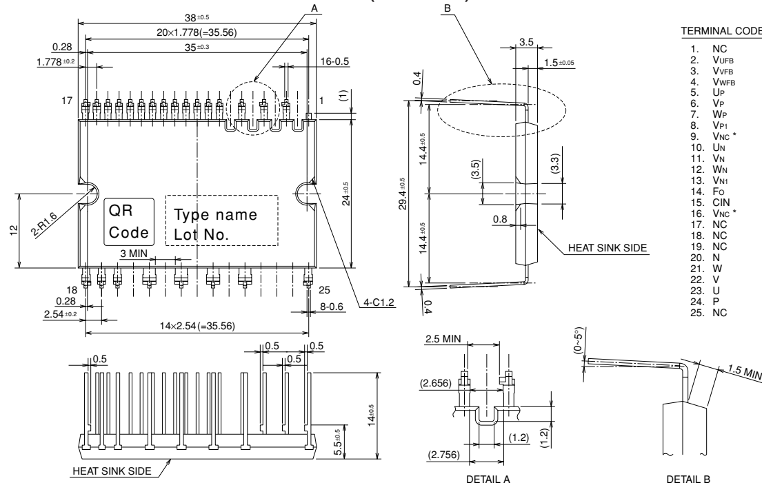
Fig. 2 LONG TERMINAL TYPE PACKAGE OUTLINES (PS21965-AT)
