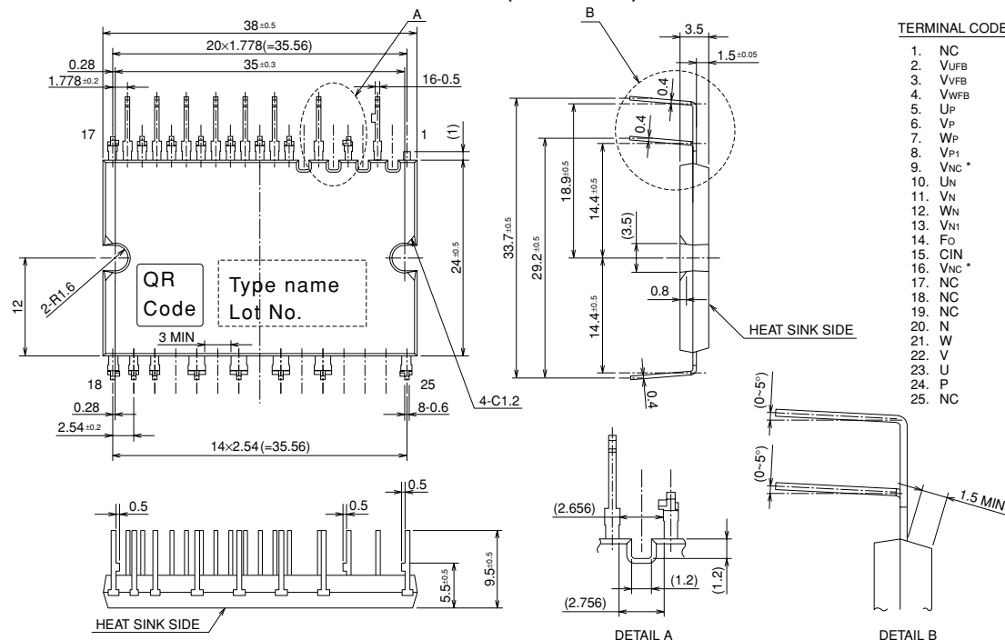
Fig. 3 ZIGZAG TERMINAL TYPE PACKAGE OUTLINES (PS21965-CT)
