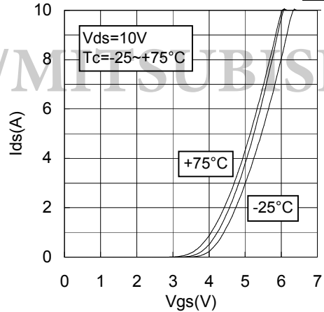
Vgs-Ids CHARACTERISTICS 2
