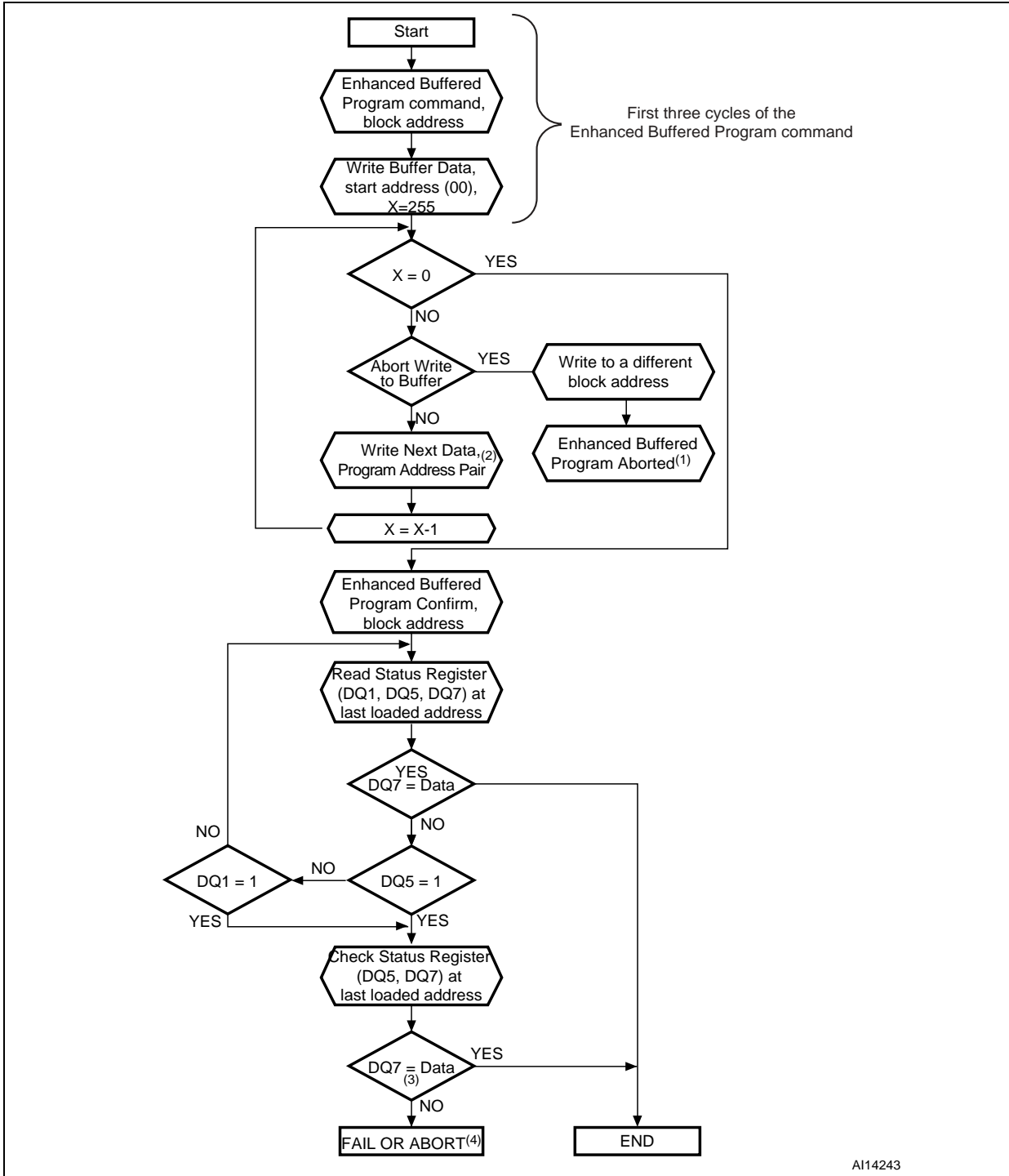
Figure 24. Enhanced buffered program flowchart and pseudocode
