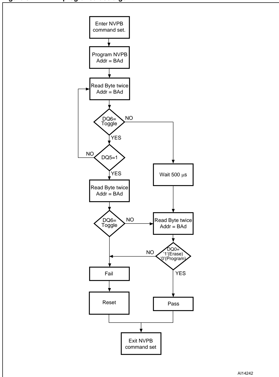
Figure 6. NVPB program/erase algorithm
