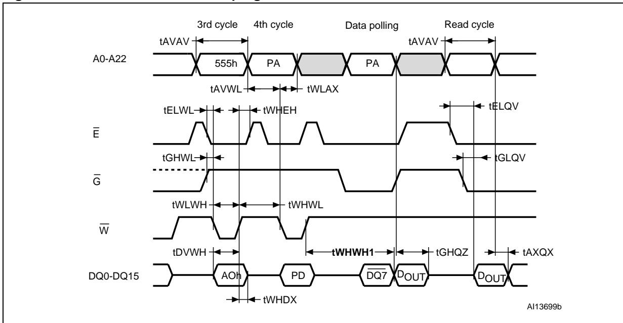
Figure 15. Write enable controlled program waveforms
