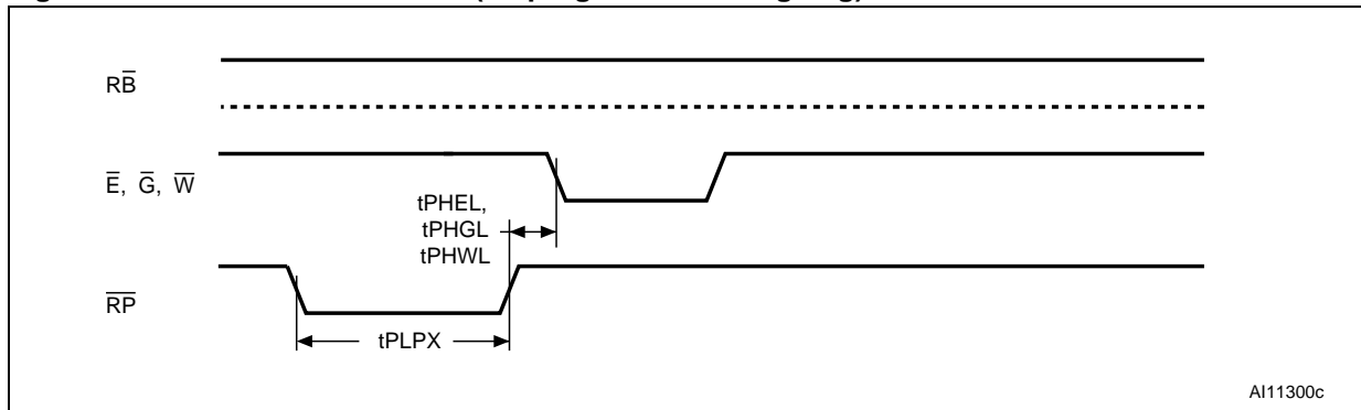
Figure 18. Reset during program/erase operation AC waveforms
