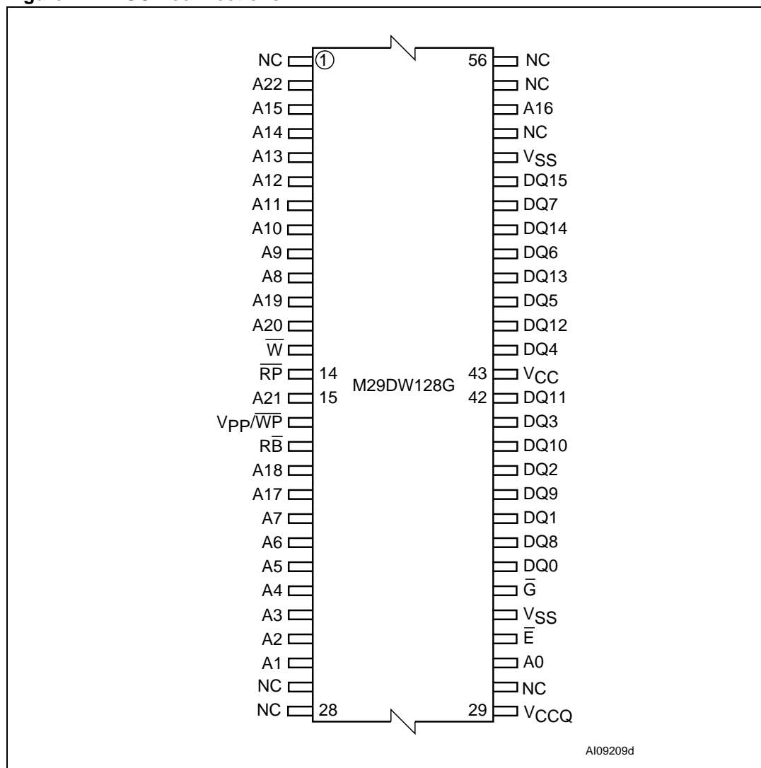
Figure 2. TSOP connections
