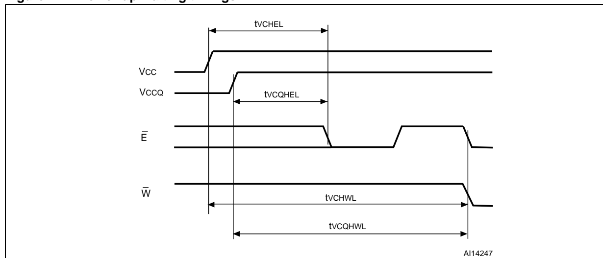
Figure 12. Power-up waiting timings
