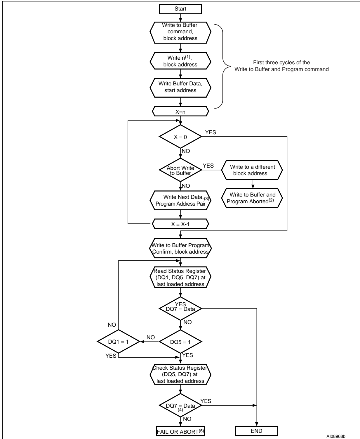
Figure 23. Write to buffer program flowchart and pseudocode
