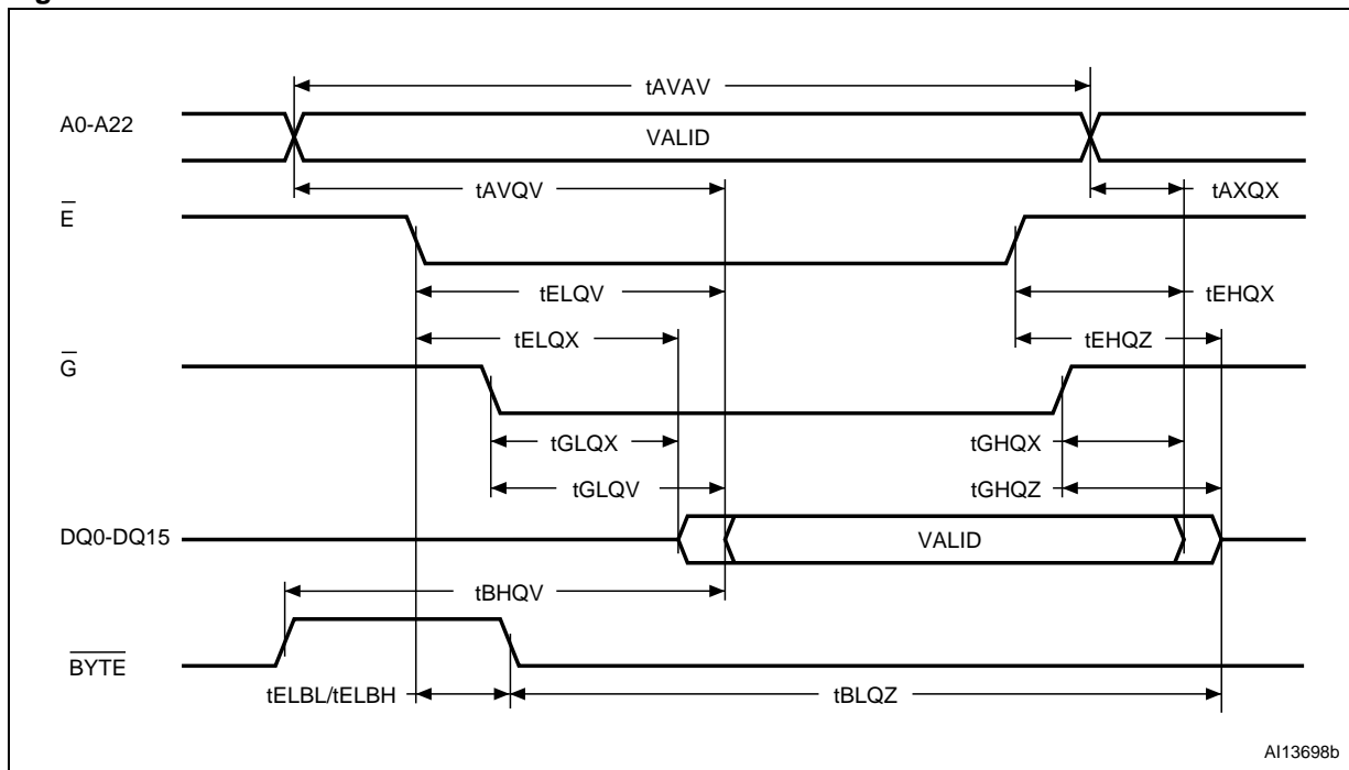
Figure 13. Random read AC waveforms
