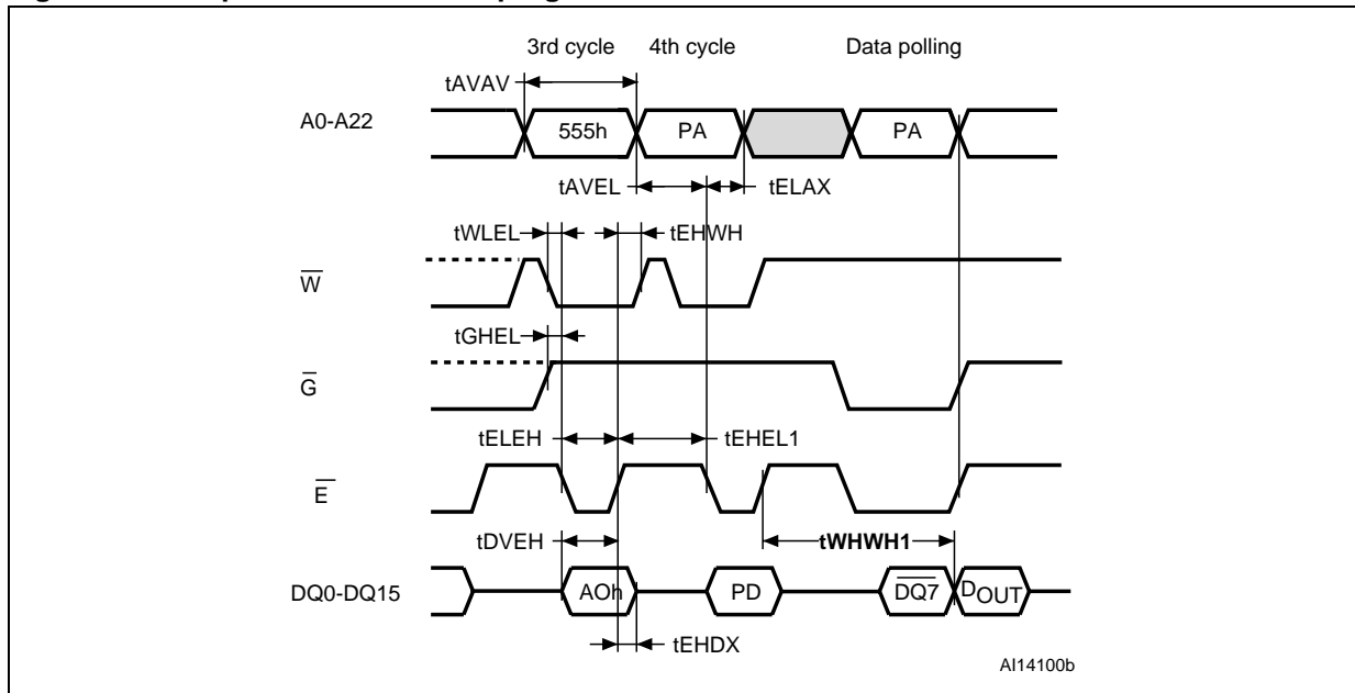
Figure 16. Chip enable controlled program waveforms
