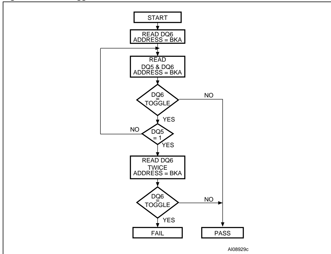
Figure 9. Data toggle flowchart
