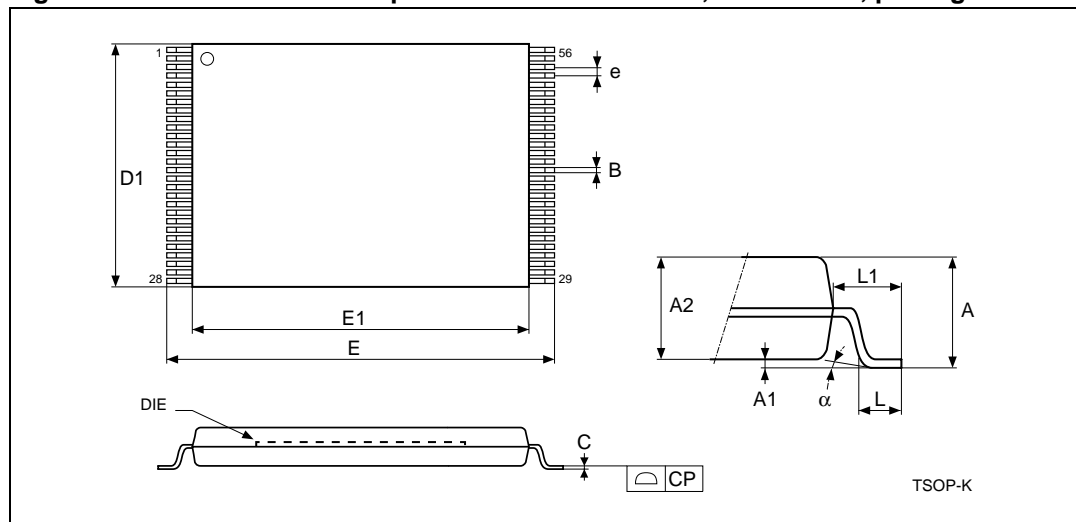
Figure 21. TSOP56 – 56 lead plastic thin small outline, 14 x 20 mm, package outline
