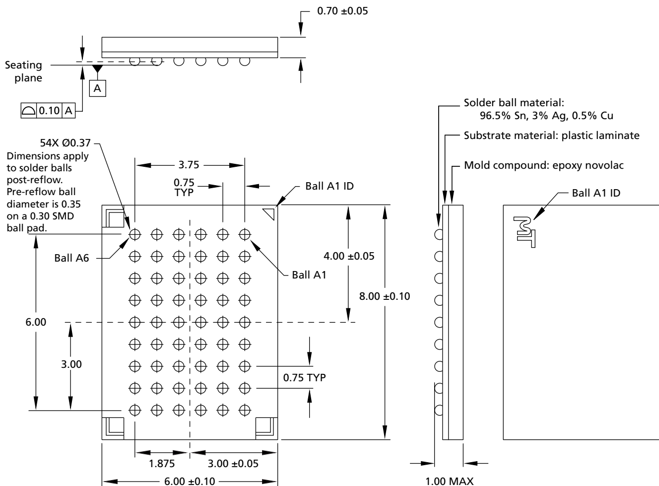
Figure 49: 54-Ball VFBGA
