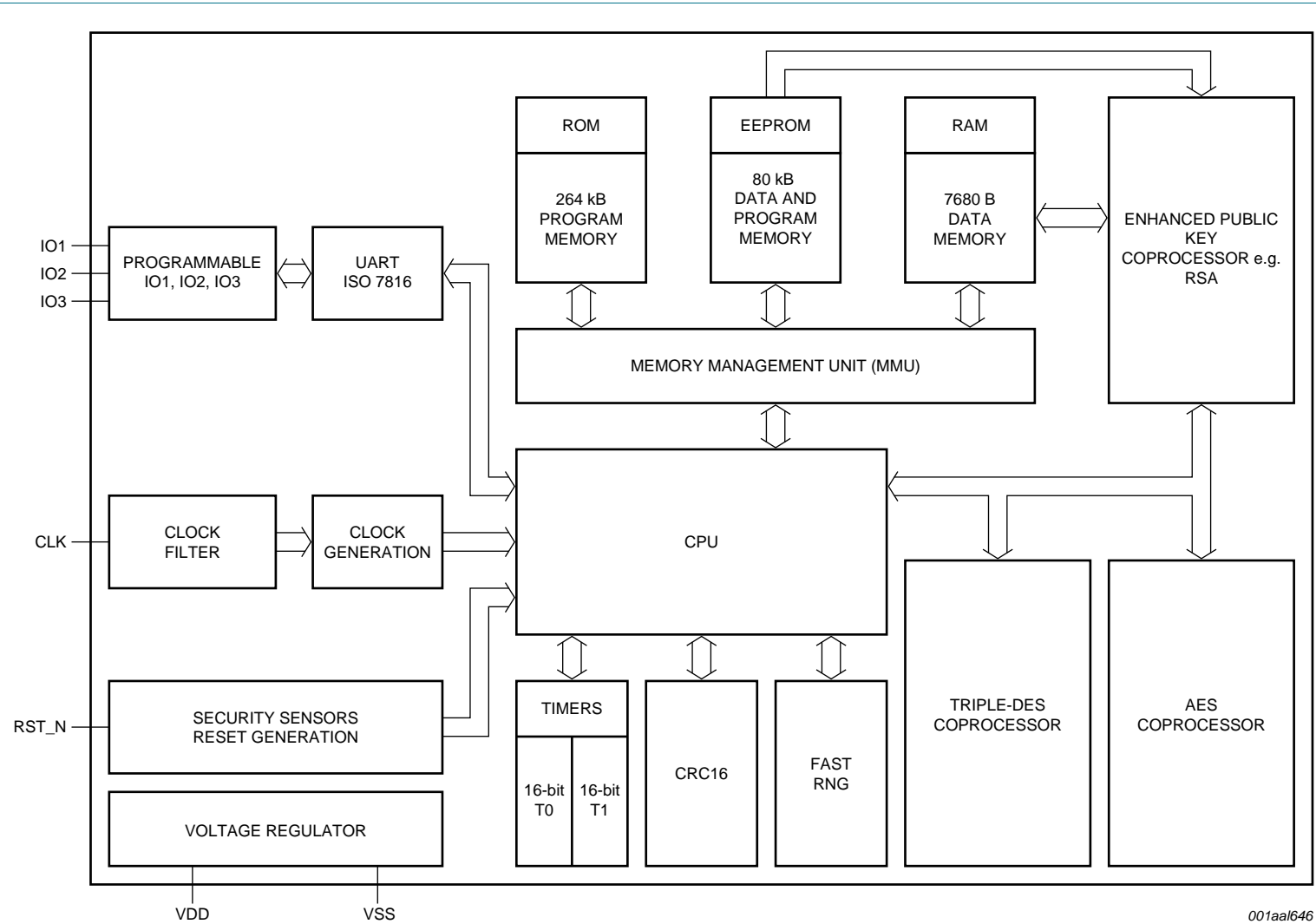
Fig 1. Block diagram
