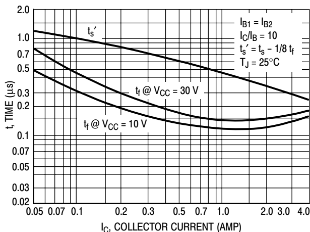
Figure 10. Turn-Off Time
