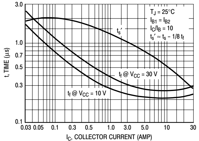
Figure 8. Turn-Off Time
