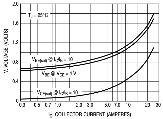
Figure 13. "On" Voltages
