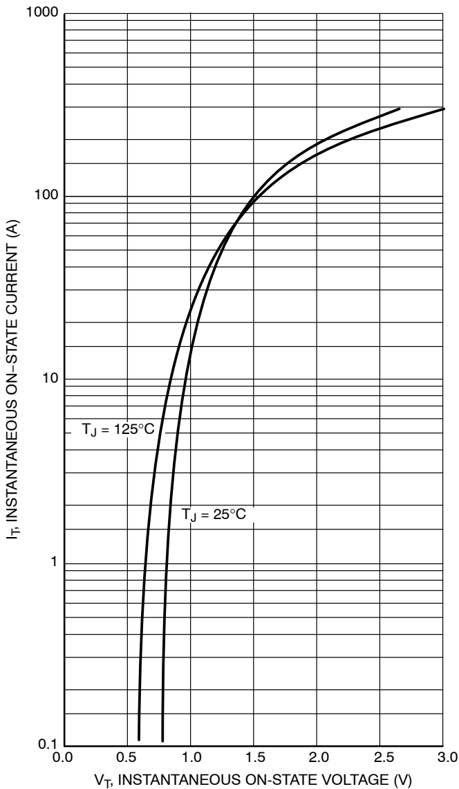
Figure 3. On-State Characteristics
