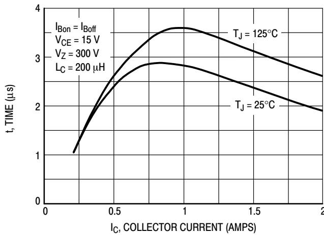
Figure 15. Inductive Storage Time, t_s @ h_{CE} = 5
