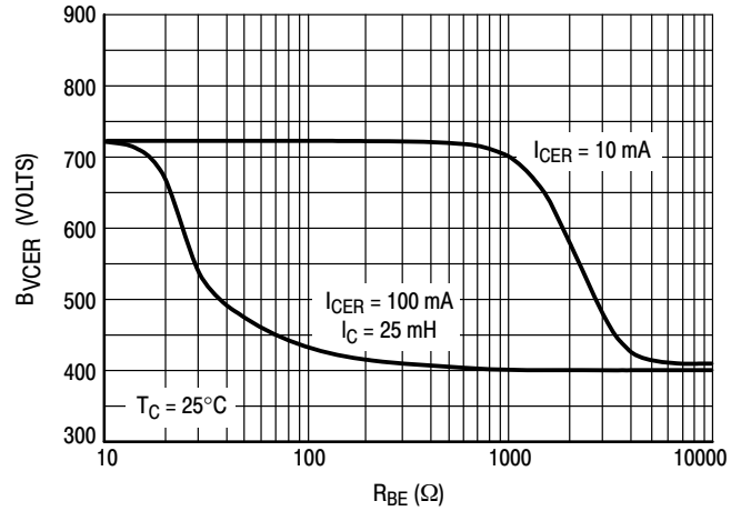
Figure 12. V_{CER} = f(R_{BE})
