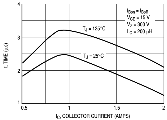
Figure 16. Inductive Storage Time, t_s @ h_{CE} = 10
