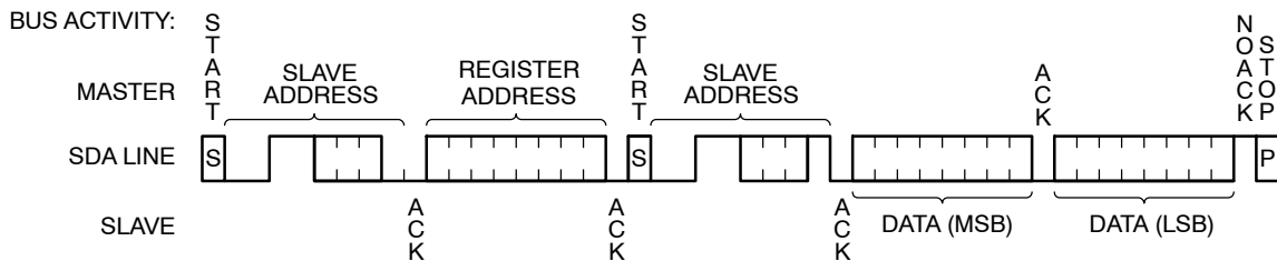
Figure 14. Selective Read
