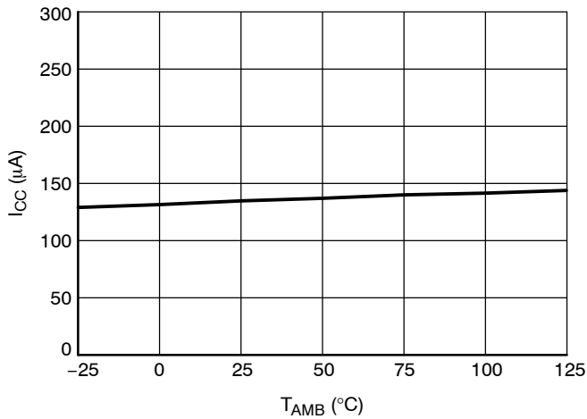
Figure 2. Active Current (I 2 C-bus Idle)
