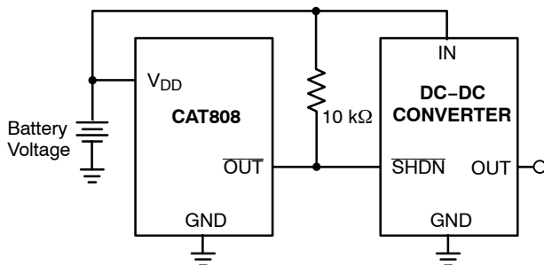
Figure 1. Typical Application
