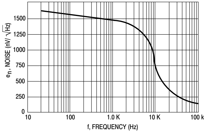
Figure 12. Noise Voltage
