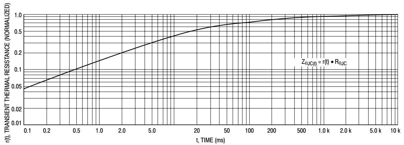
Figure 8. Thermal Response
