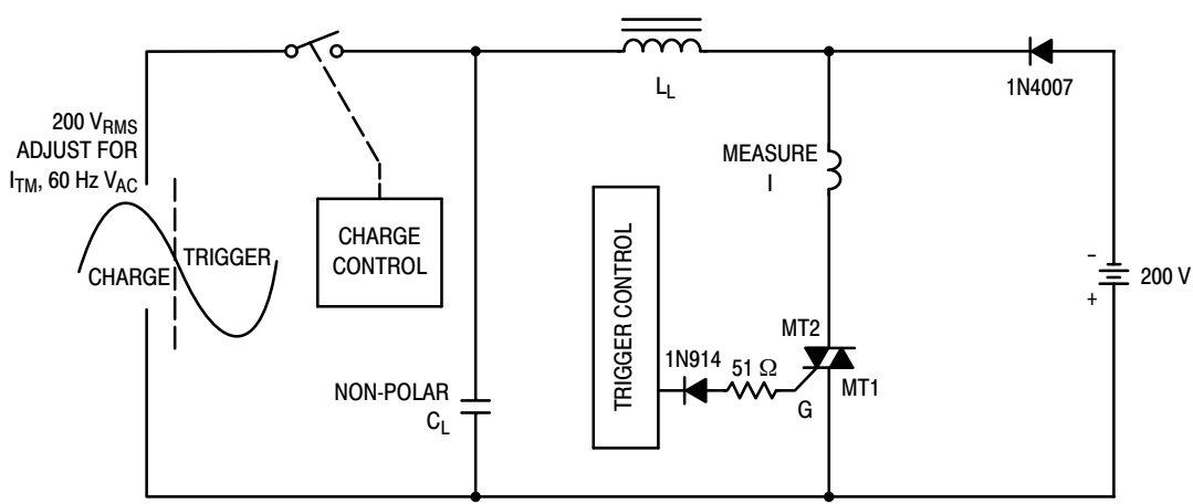
Figure 16. Simplified Test Circuit to Measure the Critical Rate of Rise of Commutating Current (di/dt)_c
