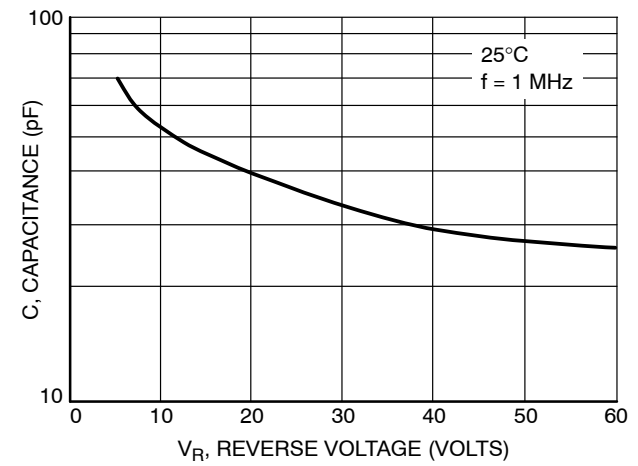
Figure 4. Typical Capacitance
