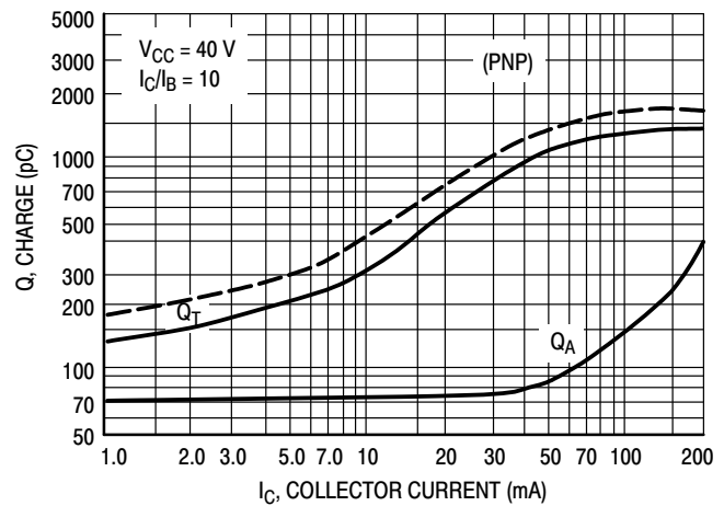
Figure 23. Charge Data
