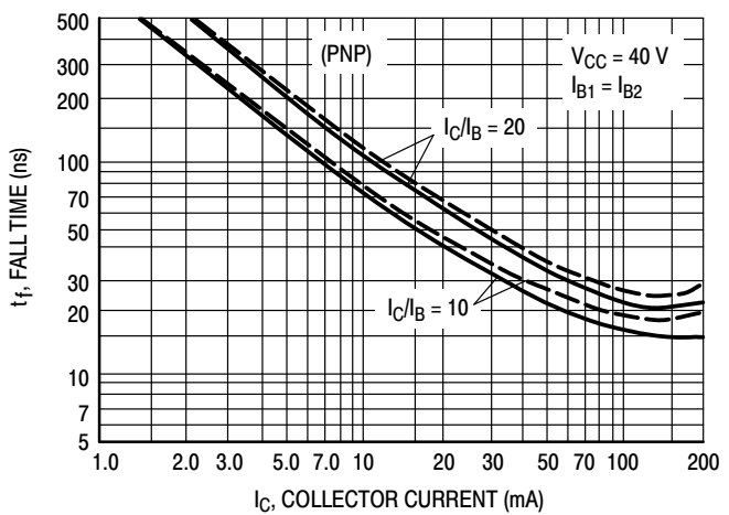
Figure 25. Fall Time
