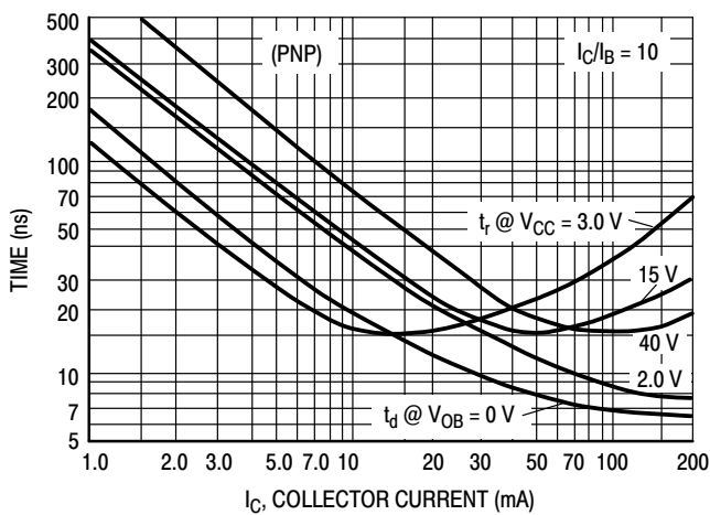
Figure 24. Turn-On Time
