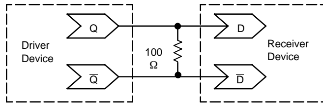
Figure 3. Typical Termination for Output Driver and Receiver Evaluation
