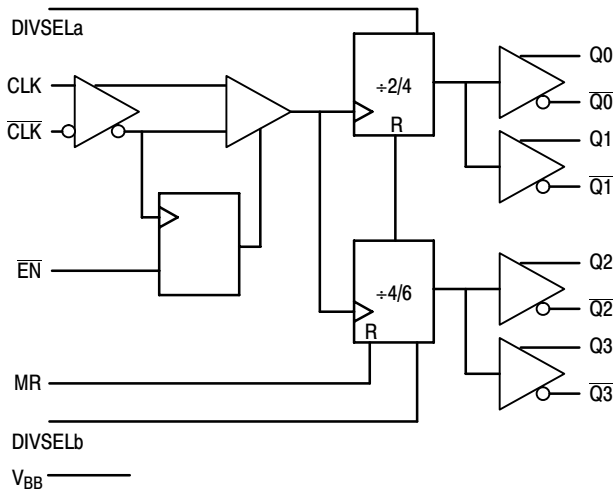
Figure 2. Logic Diagram
