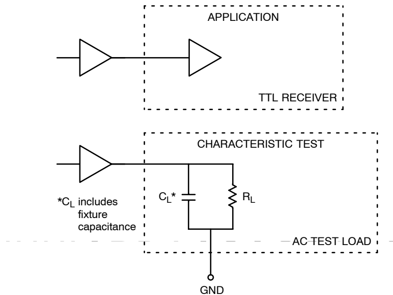
Figure 1. TTL Output Loading Used for Device Evaluation
