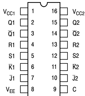
Figure 2. Pin Assignment
