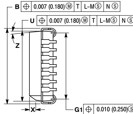
VIEW D-D
