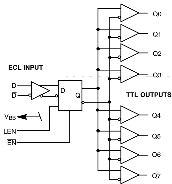
Figure 2. Logic Diagram
